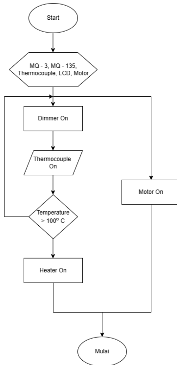
Figure 3. Flowchart
