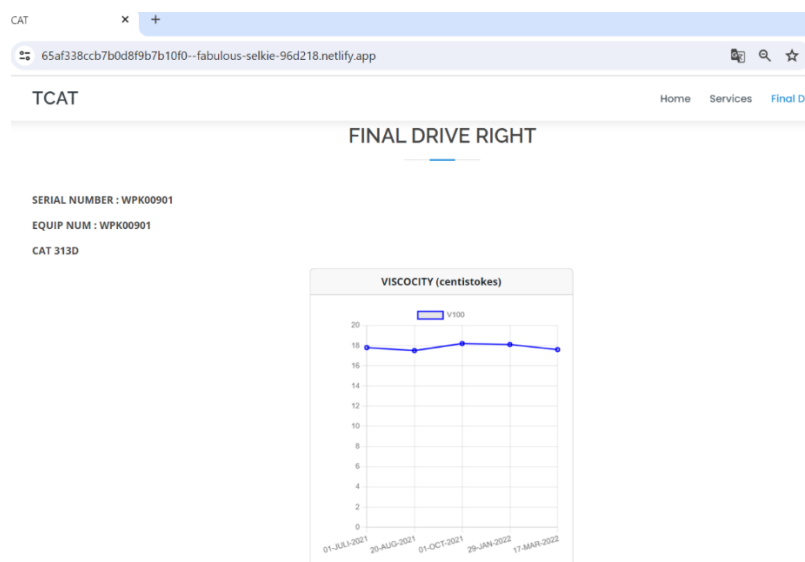
Figure 6. Viscosity Chart
