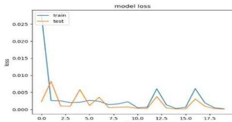
Fig. 5. Loss for Dataset-A
