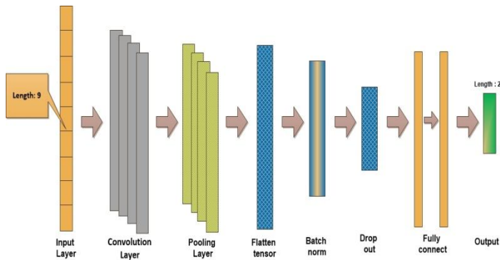
Fig. 2. 1D CNN architecture
