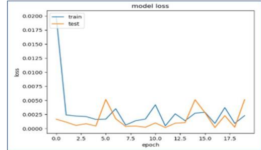
Fig. 7. Loss for Dataset-B
