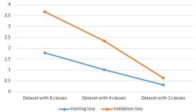
Fig. 6 Visualization of the training and validation loss between the three experiments.
