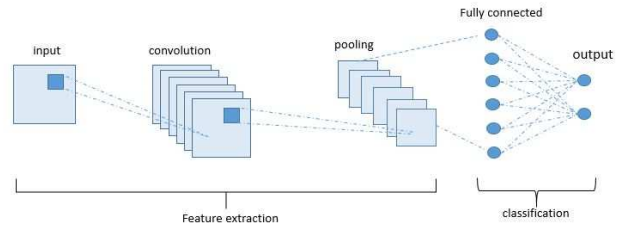
Fig. 3 The basic architecture of CNN algorithm.
